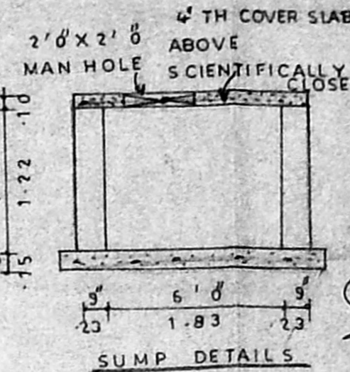
SUMP DETAILS
