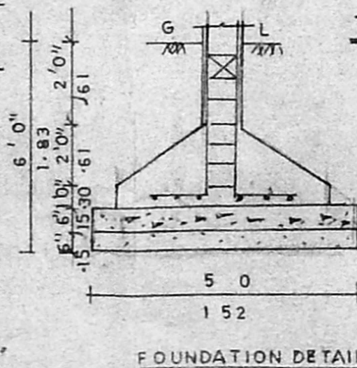
FOUNDATION DETAIL
